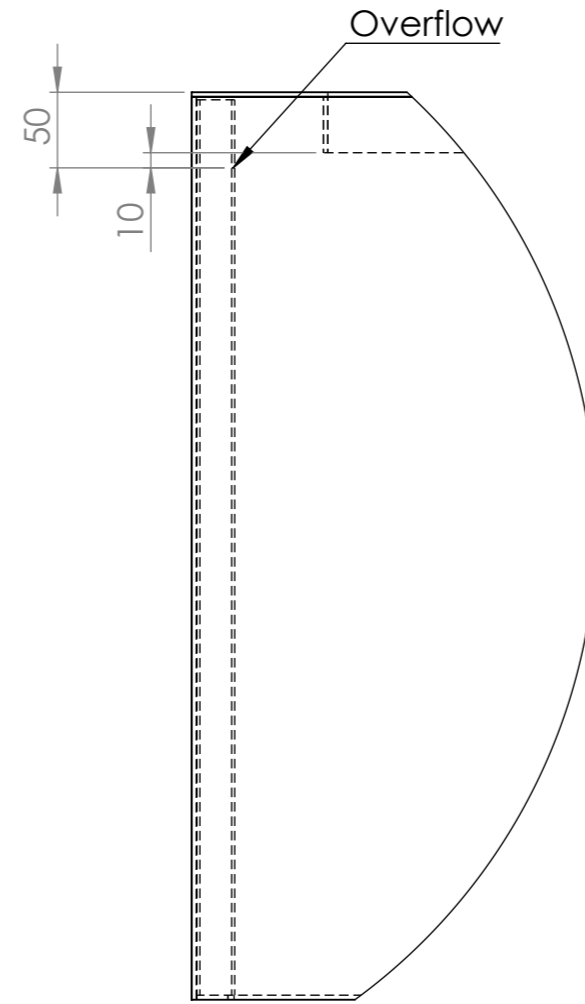
DETAIL C SCALE 1 : 5
